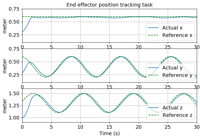
FIGURE 4.4: Experiment A: tracking plot for the MPC scheme with Riccati gains. Tracking weights are two times higher than in Fig. 4.3 (50 instead of 25).
