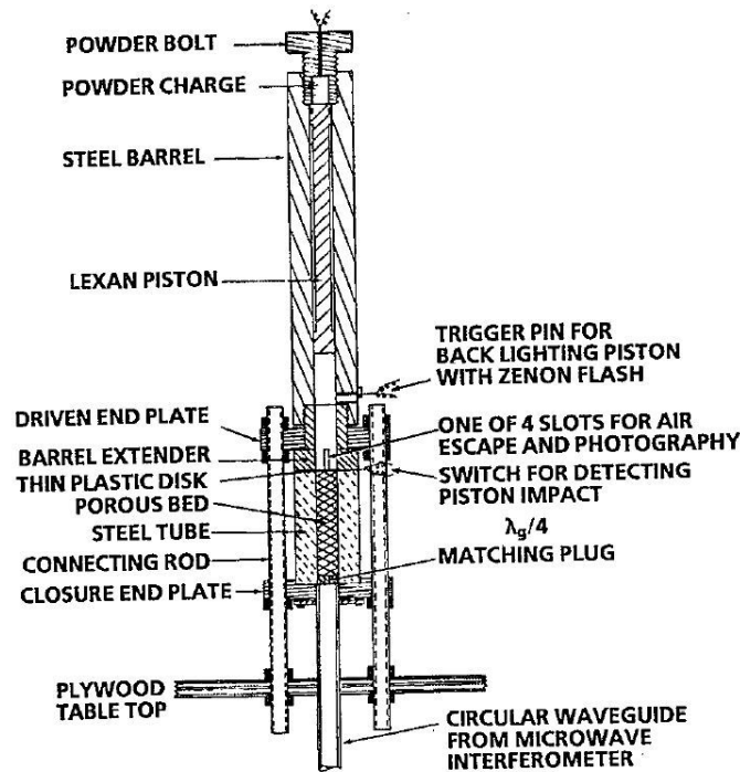
FIGURE 1.25 – Montage expérimental de KRALL et al. [77]
