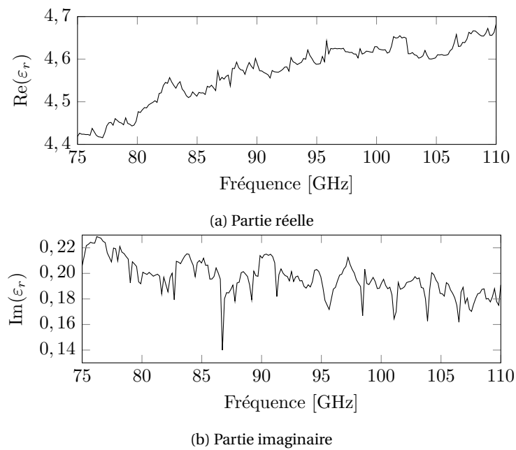
FIGURE C.11 – Permittivité complexe du mélange RDX-Aluminium-Liant inerte
