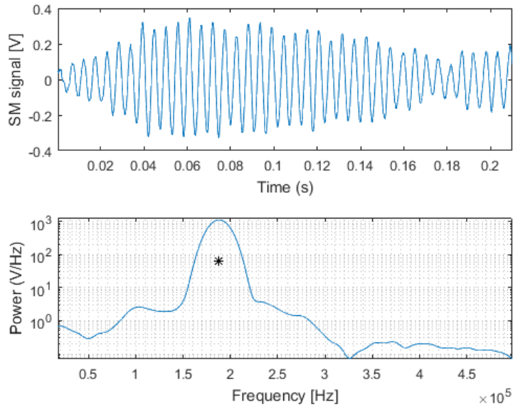
Figure 3.13: Visualization of weighted moment calculation on section of SM signal. Top plot: SM signal plotted in blue. Bottom plot: Power spectrum of the SM-signal. The average frequency \bar{f} = 188 kHz, is marked with a star.
