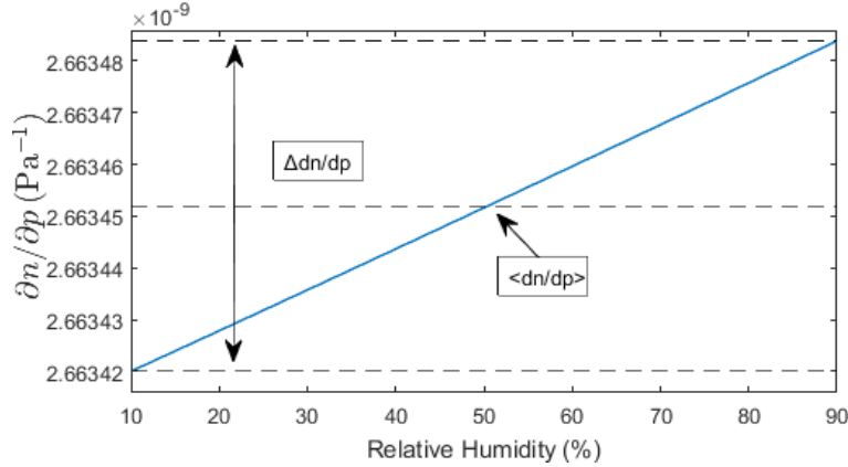
Figure 2.10: Change in \frac{\partial n}{\partial p} at varying relative humidity RH at temperature T \sim 19^\circ\text{C} and pressure p \sim 89 kPa.
