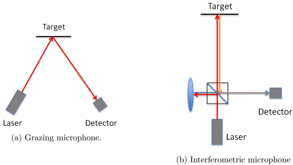
Figure 1.4: Laser microphones recording movement of distant vibrating diaphragm.
