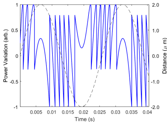
Figure 1.18: Simulation of laser signal (blue line). The laser measures a target moving sinusoidally with frequency of 40 Hz and amplitude 2 \mu\text{m} zero to peak (black line). C = 2.5 and l_{ext} = 30\text{cm}
