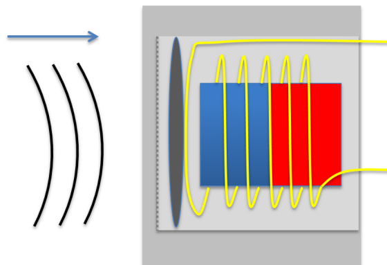
Figure 1.2: Dynamic Microphone with a diaphragm attached to a coil that is wrapped around a magnet. Pressure waves coming in from the left.
