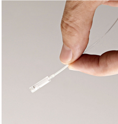
Figure 1.3: Optical Fiber Microphone [4], [5] where light reflected from the diaphragm is used to register audio signals.
