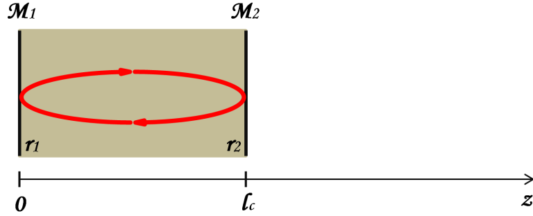
Figure 1.14: Schema of Fabry-Perot Laser Cavity
