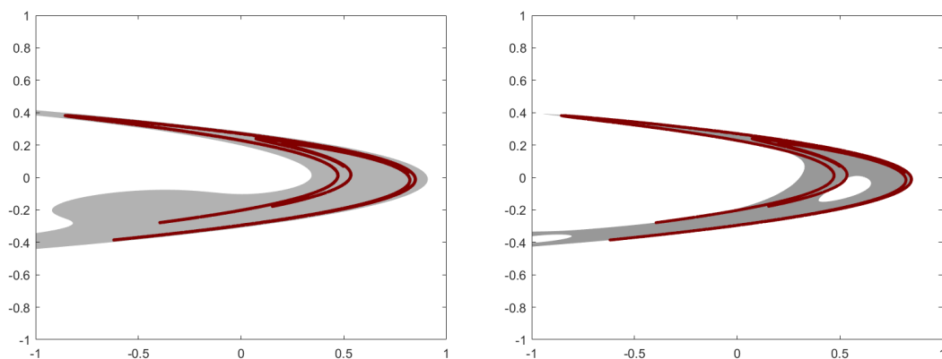
Figure 5.5: Outer approximations (gray) of the attractor (red) for the Hénon map for X = [-1, 1]^2 . Left: approximation, degree 6 polynomials and \beta = -\log(0.002) , \gamma = 0.05 . Right: Intersection of approximation by degree 8 polynomials obtained by different values \beta = -\log(0.001), -\log(0.002), -\log(0.01) and \gamma = 0.002, 0.05, 0.2 .
