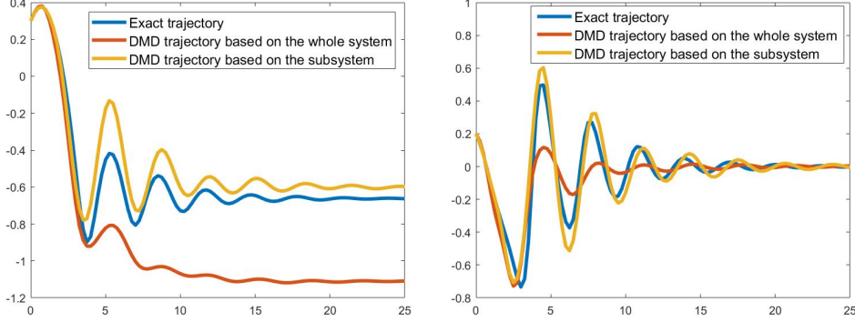
Figure 6.6: DMD approximations based on the whole system and on the subsystem induced by I = \{1, 2, 5, 6\} for (6.58) with initial value x_0 = (-0.3, -0.3, 0.7, 0.5, 0.3, 0.2) , trained on the same data with randomly generated 1000 radial basis functions. Left: DMD approximation for x_1^3 , right: DMD approximation for x_2^3 .
