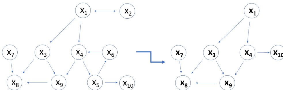
Figure 4.4: Example of a sparsity graph (left) and its condensation graph (right). The strongly connected components are C_1 = \{x_4, x_5, x_6\}, C_2 = \{x_1, x_2\} . The graph on the right arises from the sparsity graph (left) by contracting each of the strongly connected components C_1 and C_2 .
