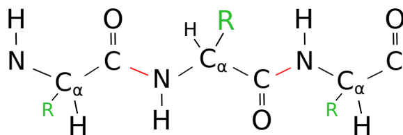
Figure 1.1: Simplified representation of a polypeptide. Peptide bonds, backbone atoms and side chains are marked in red, black and green respectively.
