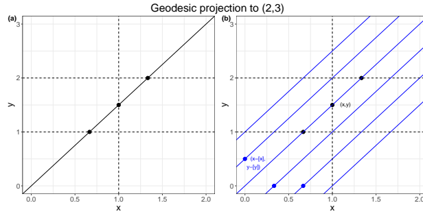
Figure A.2: First steps of the projection algorithm for the closed geodesic corresponding to the straight line of director vector u = (2, 3) . The three points in black constitute the ensemble \mathcal{P}_u . In (b), points of \mathcal{P}_u are transferred to [0, 1] \times [0, 1] by subtracting to their coordinates their integer parts. The blue lines are the elements of \mathcal{L}_u .
