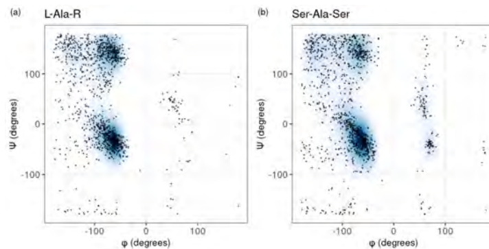
Figure 3.3: (a) Sample and kernel density estimate of alanine (\phi, \psi) distribution when the identity of its left and right neighbor is not taken into account. (b) Sample and kernel density estimate of (\phi, \psi) distribution corresponding to tripeptide Ser-Ala-Ser (a fragment of the three consecutive amino-acids serine, alanine, serine).
