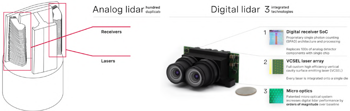
Figure 2.14: Comparison between analog and digital LiDAR architectures, excerpt from [38].
