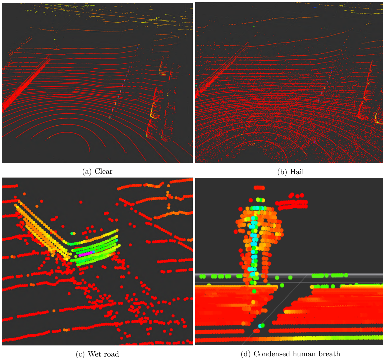
Figure 6.4: DVE scenarios cause false positive points in the point clouds.
