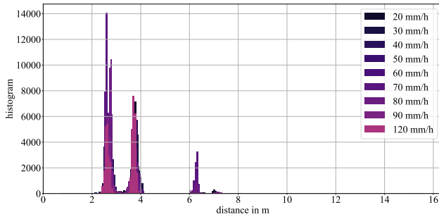
(a) VLP-32
