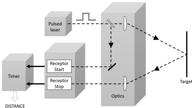
Figure 2.30: Schematic representation of a direct ToF processing chain, excerpt from [62].
