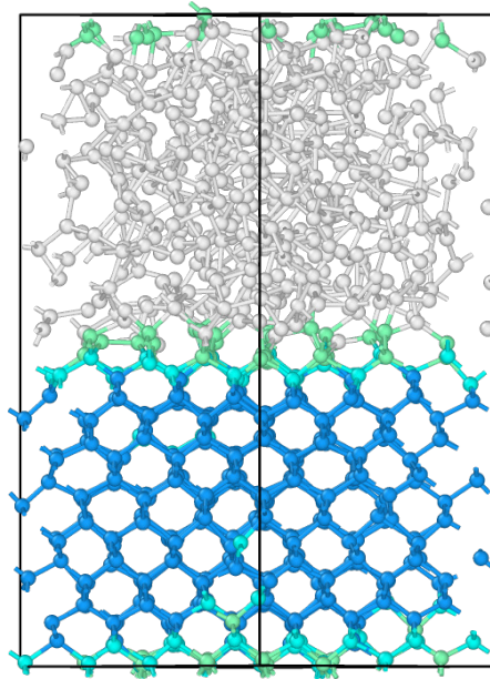
Figure 41: Example of a representative sample to study the melting temperature. Colors are obtained with the Maras et al. descriptor[142] and highlight the perfect diamond structure in blue, the first and second order coordinated diamond structure in light blue, and the only first neighbor tetrahedrally coordinated in green. White atoms are randomly arranged in a liquid phase. This particular configuration is a 4x4x8 cell.
