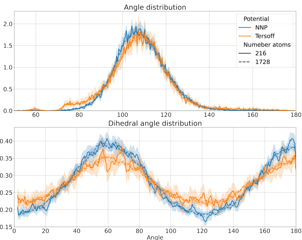
Figure 28: Angular distribution (top panel), and dihedral distribution (bottom panel) for the NN potential and and Tersoff [38] potentials, and different numbers of atoms. For each potential increasing the number of atoms only smooths the curves thanks to the increased sampling. The features in the dihedral angle distribution shows the existence of a medium-range order, up to second nearest neighbors, more pronounced for the NN potential.
