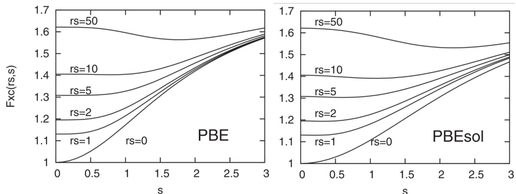
Figure 8: Enhancement factors of PBE and PBESol, for spin-unpolarized systems, as a function of the reduced density gradient, for various values of r_s , from [48].
