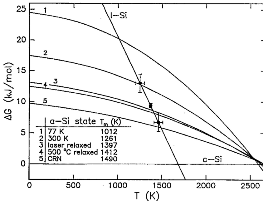
Figure 3: Reproduced from Ref. [11]. Calculation of the Gibbs free energy of l-Si and various states of a-Si relative to c-Si. The curves are theoretical estimates and the listed melting temperatures T are derived from the intersection of the free energy curves of a-Si with the one of l-Si. Parameters used in the theoretical model to obtain the curves have been obtained from samples with a thermal history specified in the inset. Continuous random network (CNR) is a theoretical defect-free a-Si structure. Points refer to experimental estimates performed on a-Si with different degrees of relaxation. Higher points are un-relaxed samples, while lower points are relaxed samples.
