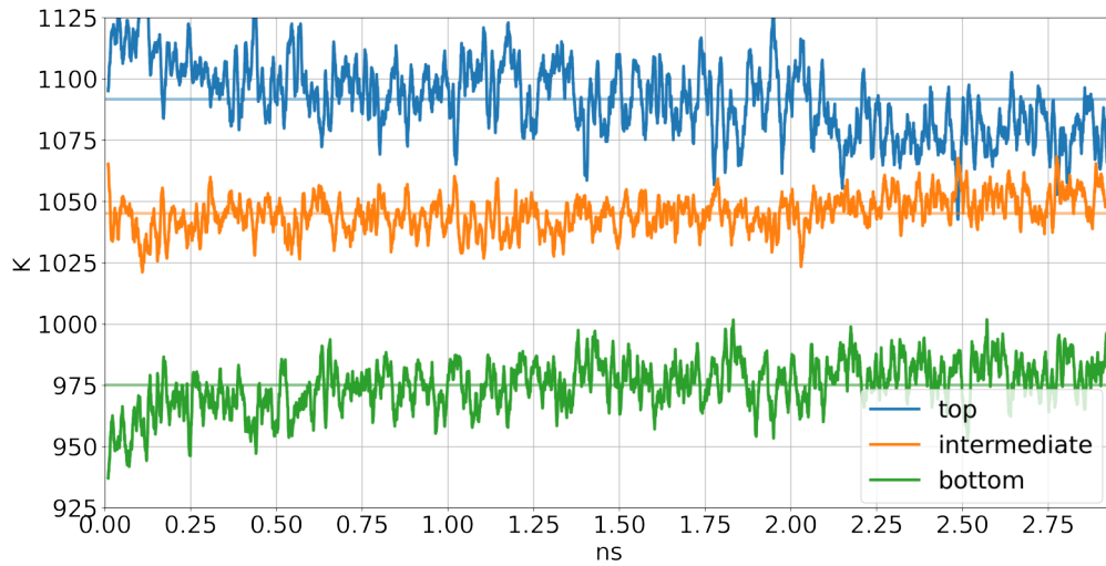
Figure 37: Temperature in the different regions for the case of the 2560k atoms as a function of time in the simulation targeted at 1050K previously presented in figure 34. In the beginning, we can see that the 180 ps equilibration phase is common to all regions. In the middle, the period of time deemed valid for the reconstruction has constant temperatures in all the regions, especially at the interface where relevant phenomena are happening. In the end, after 1.7 ns once the sample has crystallized no more energy is released by the phase transition, and the surface cools down.
