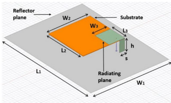
Fig. 1. Configuration of the antenna with single PIFA.
