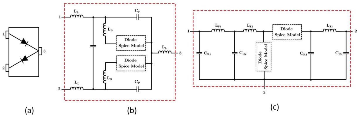
Figure II.5. SOT-23 Package Circuit models of the Schottky diode: (a) General Package style; (b) Model by HP Inc.; (c) Model by Skyworks (SK).
