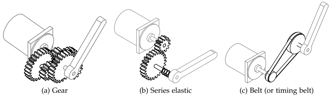
Figure 15: Transmission types
