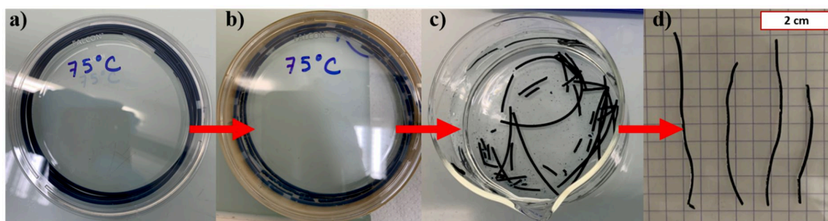
Figure 4.5: Preparation steps of the PEDOT:PSS/PAAc double network gel. Images of a) the gellified PEDOT:PSS dispersion injected in the PP tubing, b) PEDOT:PSS gel after heating at 75°C for 1 h, c) PEDOT:PSS gels soaked in the AAc monomer solution and d) PEDOT:PSS/PAAc DN gels with average swollen diameter of 1.6 mm after polymerization of the AAc monomers.
