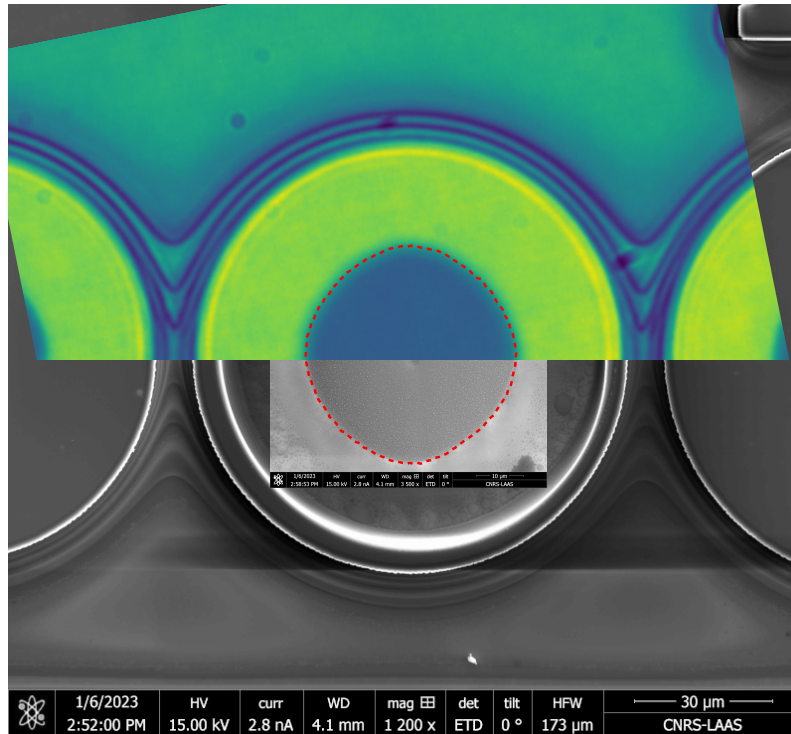
Figure 3.36: Composite image with top to bottom overlap of the in-situ inspection view obtained with shaped spectrum illumination (clipped, with green colormap), the zoomed FIB etching SEM image (light gray), the overview FIB etching SEM image (darker gray). The red dashed line corresponds to the aperture fitted using the shaped spectrum illumination. Taken from [58].
