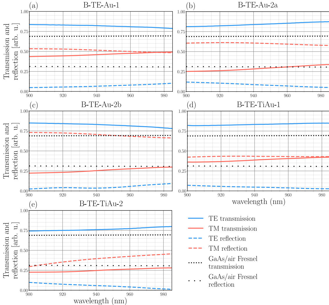
Figure 2.28: Spectroscopy measurements of fabricated B-TE configurations at normal incidence between 900 and 985 nm.
