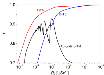
Fig. 14. Transmittance as a function of sheet resistance for B-TE (blue), T-TM (red) and the Au-grating-TM (black) calculated for \lambda = 1 \mu\text{m} .
