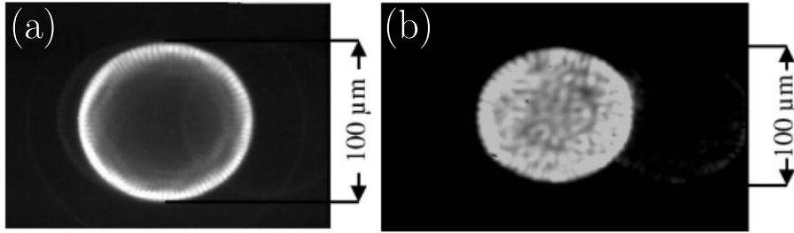
Figure 1.4: Near-field intensity distribution in a 100- \mu\text{m} oxide aperture (a) top-emitting VCSEL, and (b) bottom-emitting VCSEL. Taken from [5].
