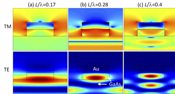
Fig. 7. Distributions of optical field intensity within a single period of T_{op} at three different wavelengths (in columns) illuminated by TM and TE polarizations (in rows).
