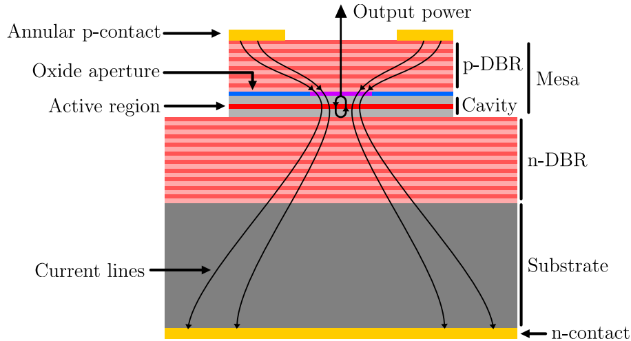
Figure 1: Cross-section of a standard oxide-confined top-emitting VCSEL.
