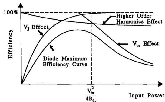
Figure II.2. General relationship between the RF input power and the conversion efficiency.
