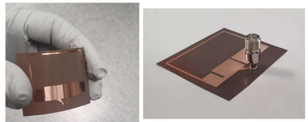
Fig. 8. Photo of the manufactured antenna in cleanroom and with U.FL connector and SMA adaptor mounted.
