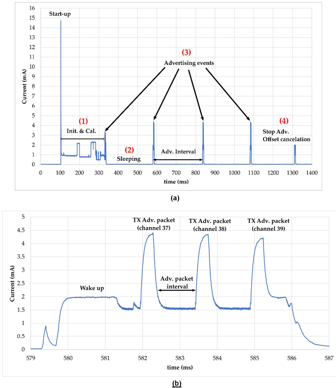
Figure III.16. (a) Current consumption profile of the BLE SN during broadcasting obtained with the power measurement tool of MCUXpresso IDE software; (b) Current consumption profile of the BLE SN during an advertising event.
