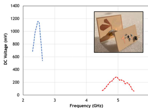
Figure VII.1. Dual -Band Rectenna : Measured harvested dc voltage of the rectenna across a 10 k \Omega for an estimated received power of -2.2 dBm (low band) and -7 dBm (high band). The inset shows a photo of the prototyped rectenna.
