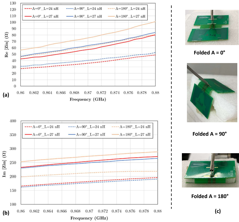
Figure V.14. The measured input impedance of the loaded UHF antenna on different folded angle ( 0^\circ correspond to the flat position) : (a) Real part of the input impedance of the characterized antenna; (b) Imaginary part of the input impedance of the characterized antenna; (c) Photo of prototyped antenna under test.
