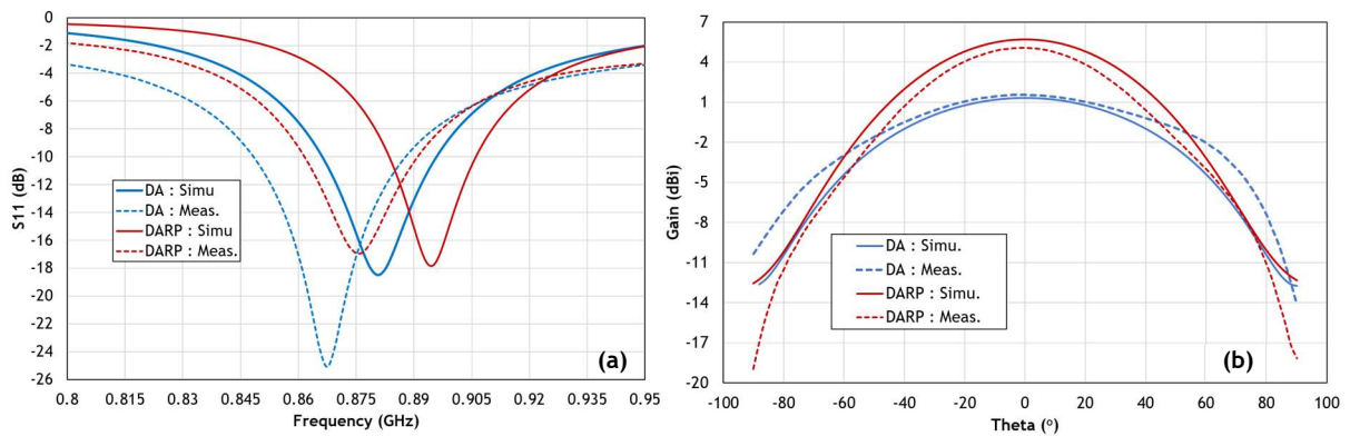
Figure III.5. (a) Comparison of the simulated and measured reflection coefficient of DA and DARP antennas; (b) Simulated and measured radiation patterns (gain in dBi) of the DA and DARP antennas in the E-plane at 868 MHz.
