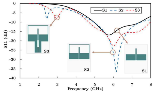
Figure 4. Simulated return loss S_{11} (dB) of the antenna at different design steps (from S1 to S3).
