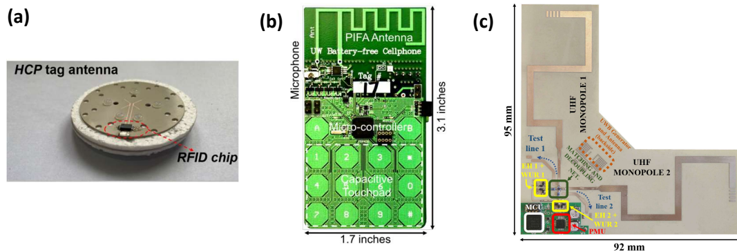
Figure I.2. Examples of developed wireless battery-free devices in the state of the art : (a) Miniaturized and Highly Sensitive Epidermal RFID Sensor for Reliable Skin Temperature Monitoring [32]; (b) First battery-free cellphone from Washington University [36]; (c) Dual-monopole UHF/UWB battery-less tag [39].
