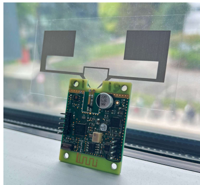
Figure III.25. Photo of the manufactured of battery-free SN prototype including a flexible antenna manufactured on transparent PET substrate operating in ISM 868 MHz frequency band.
