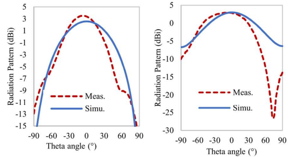
Fig. 12. Comparison of the measured and simulated radiation pattern in the E-plane (Phi = -90°) at 2.45 GHz (left) and 3.41 GHz (right).
