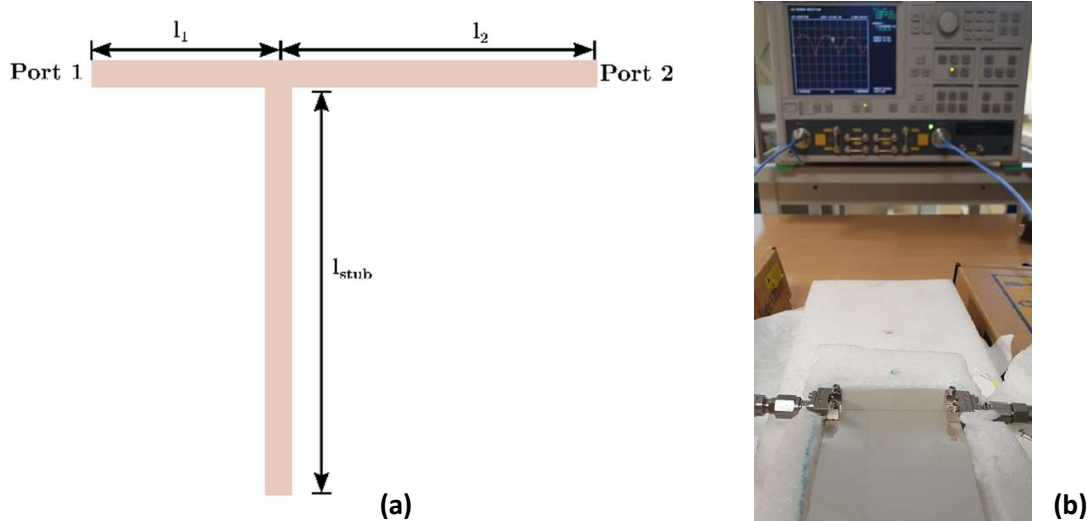
Figure IV.17. (a) Structure of the designed microstrip quarter-wavelength open-ended stud resonator ( l_1= 15 mm and l_2=35 mm; (b) Photo of the S-parameters measurement setup for the prototyped structure.
