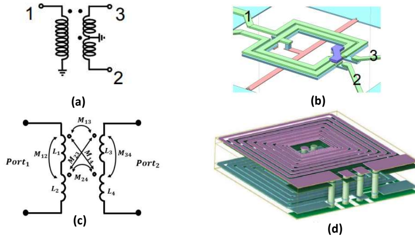
Figure IV.8. (a) Circuit model of classical transformer balun configuration simulated; (b) Image of the transformer balun simulated using Sonnet software [183]; (c) Circuit equivalent of the proposed balun using 4 layer PCB, (d) 3- D view of the balun with four-layer pattern of the stacked coil model [184].
