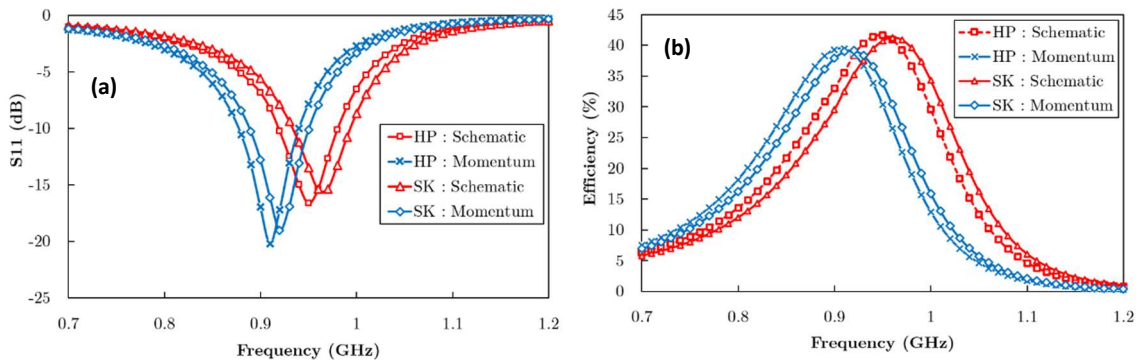
Figure II.9. Comparison between SK and HP model on schematic and Momentum simulation: (a) Return loss at -15 dBm and (b) PCE of the rectifier at -15 dBm.
