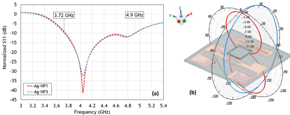
Figure VI.17. Simulation of the UWB bowtie antenna: (a) Normalized return loss for both Ag NP-based inks; (b) Radiation pattern overlay of 3D view design at 4 GHz with Ag-NP1 ink.
