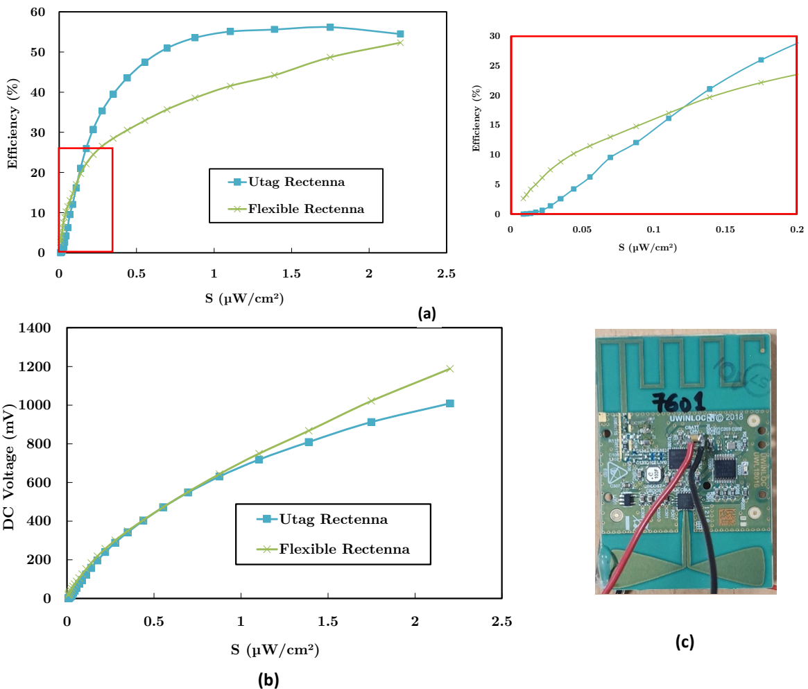
Figure IV.32. Experimental results of the comparison between the flexible rectenna R1 and the Rectenna from Uttag : (a) Conversion efficiency at 868 MHz; (b) DC output voltage at 868 MHz; (c) Photo of the modified Uttag with DC output connection across the capacitor.
