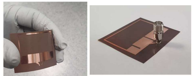
Fig. 8. Photo of the manufactured antenna in cleanroom and with U.FL connector and SMA adaptor mounted.
