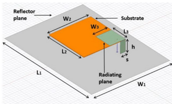
Fig. 1. Configuration of the antenna with single PIFA.
