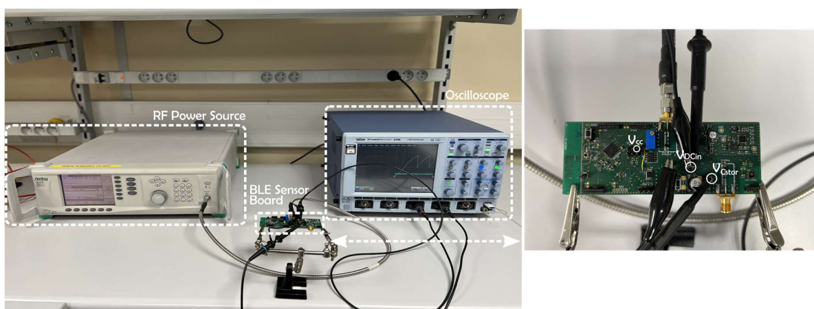
Figure III.18. Experimental setup of measuring the charging evolution of the storage capacitor.
