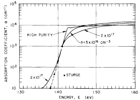
(b) For different doping levels.
