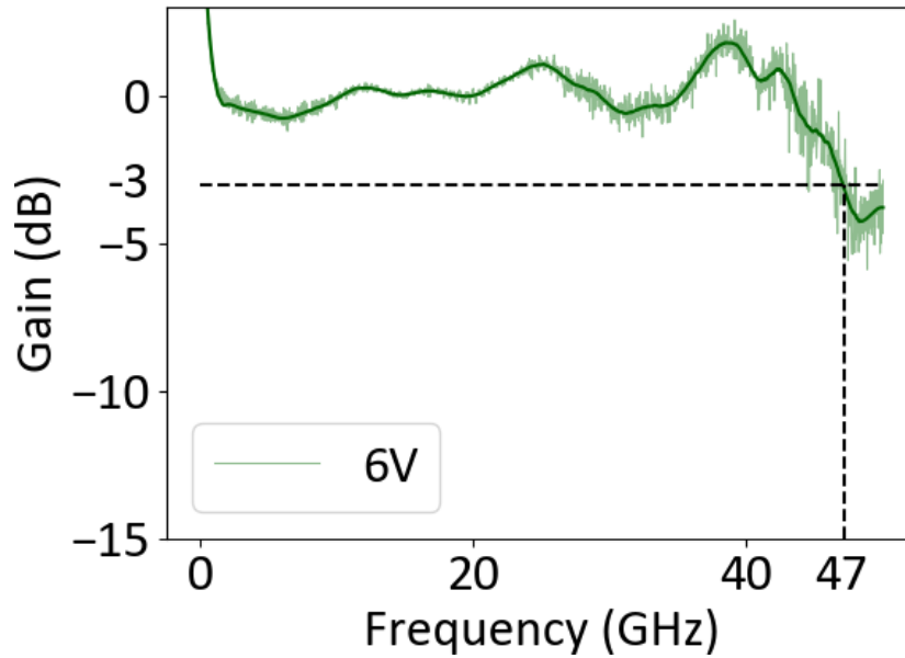
Figure 65: Voltage transfer function of the EAM with a bias of 6V.
