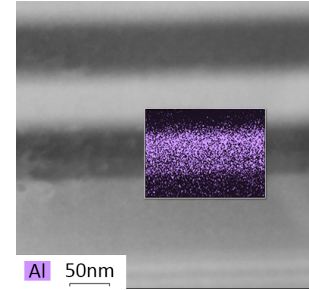
Figure 34: TEM analysis of the oxidisable aluminium layer.
