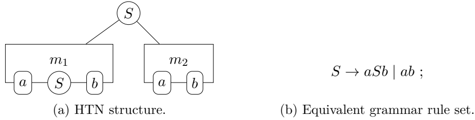
Figure 3.14: An HTN structure and the equivalent set of grammar rules.
