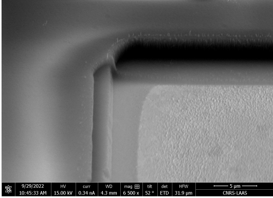
Figure 38: SEM picture of a via after BCB etching.
