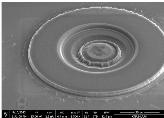
(c) EAM-VCSEL's etched double mesa with visible oxide aperture.
