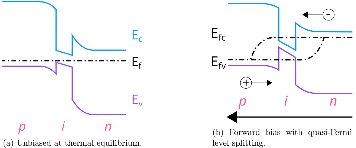
Figure 5: Conceptual Energy Band Diagram for p-i-n Junction with Quantum Well, Including Fermi Levels.
